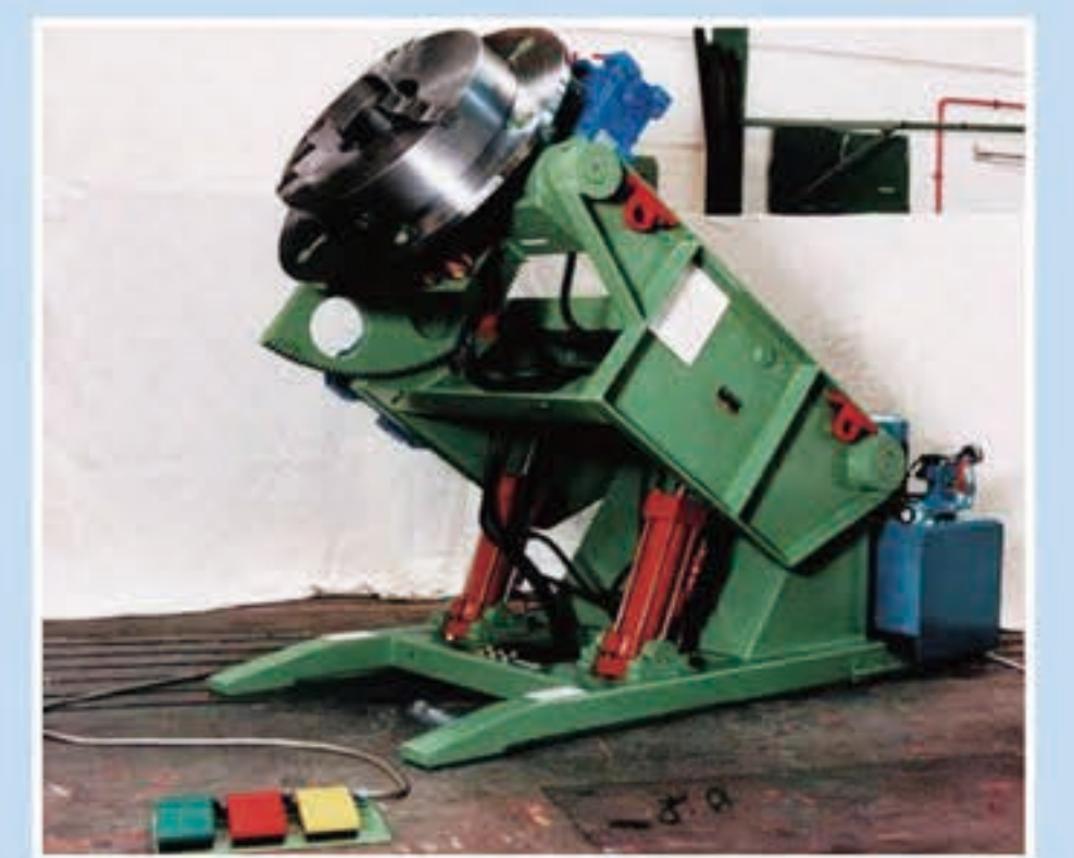
液压升降变位机 (带卡盘) Hydraulic Lifting positioner (with chuck)
